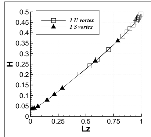
FIG. 6: Single vortex configuration.
